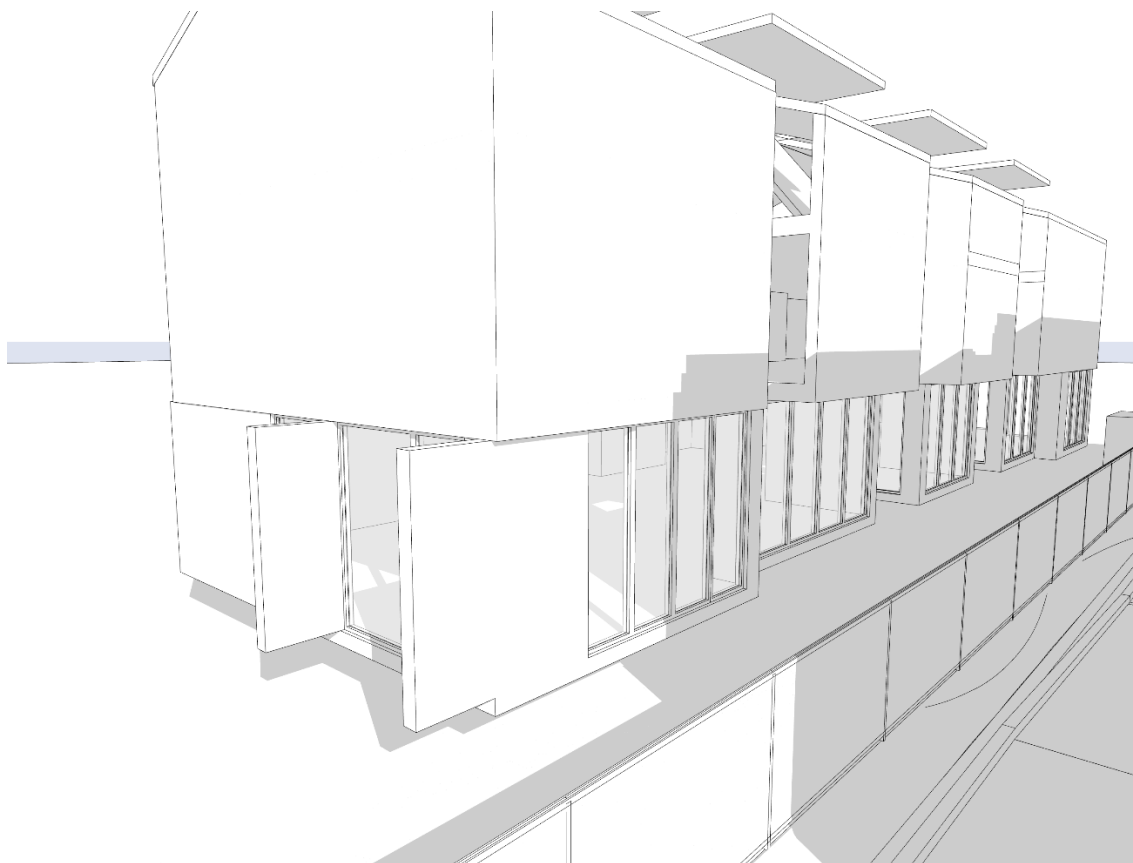
Solar analysis – Approved townhouse development at 48 Chester Avenue (front) – 11am
